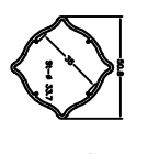
500253 Reinforcement Profile
